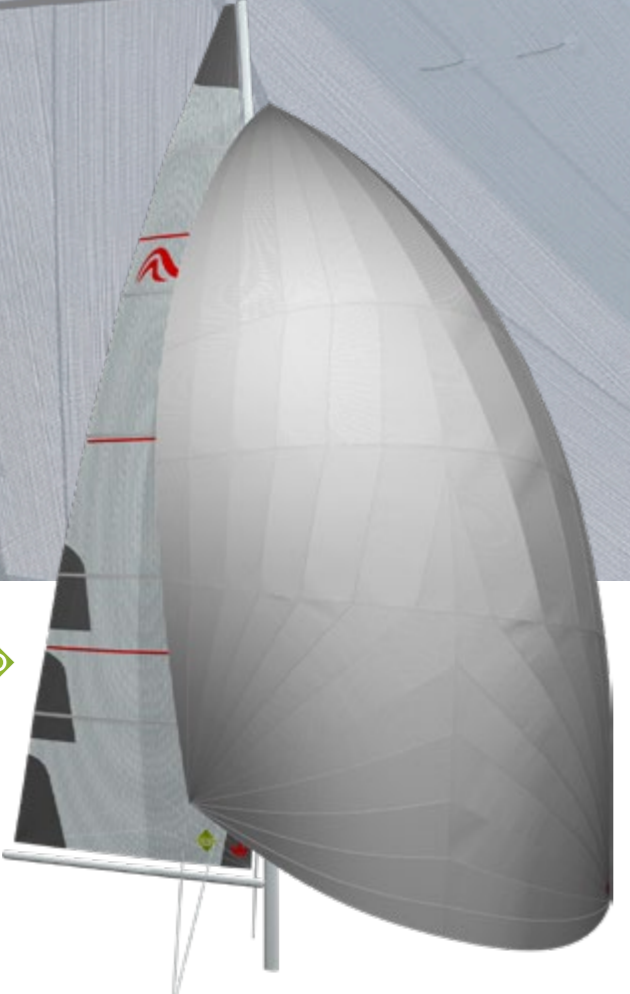
Conventional main sail Material: Elvstrøm SPS Laminate Layout: Triradial
