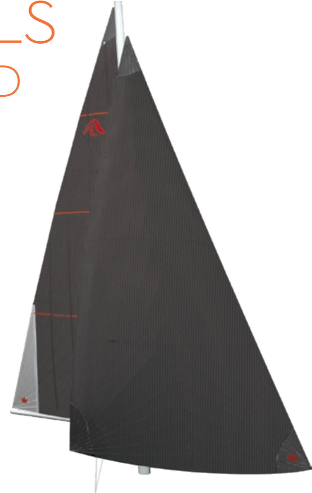
Conventional mainssail Material: Elvstrøm HPM Membrane Layout: Triradial
